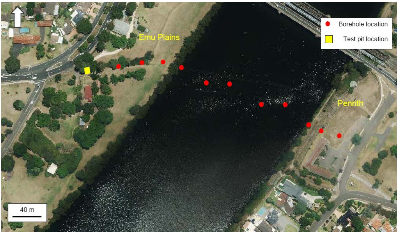
Drilling to be carried out in Nepean River at Penrith / Emu Plains
